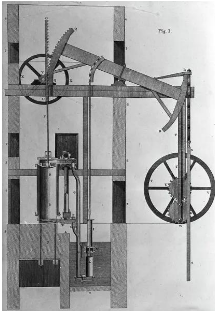
Watt's double-acting steam engine, 1769
